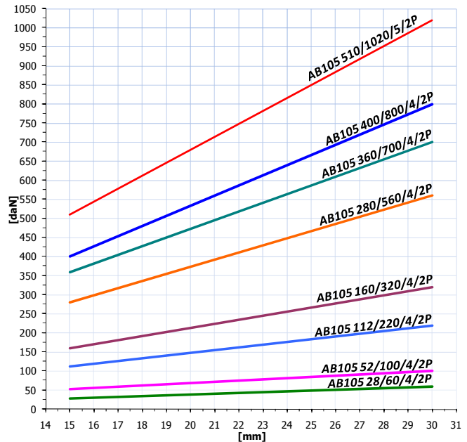
AB105...4/2P
