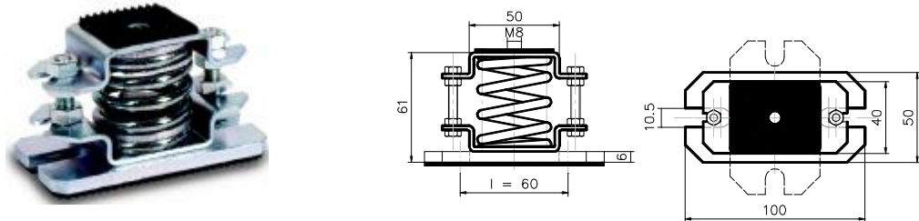
Type: 1P/AO/F
