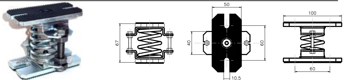
Type: 2P/AO/F
